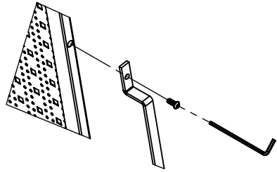
DETAIL D SCALE 2 : 15
